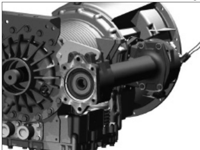
MD – Right Mounting
